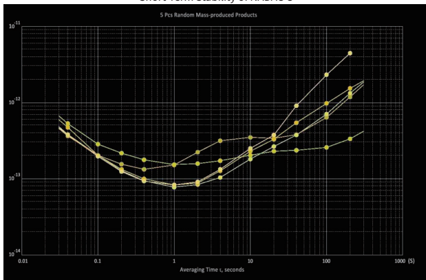
Short-Term Stability of NADAC C
