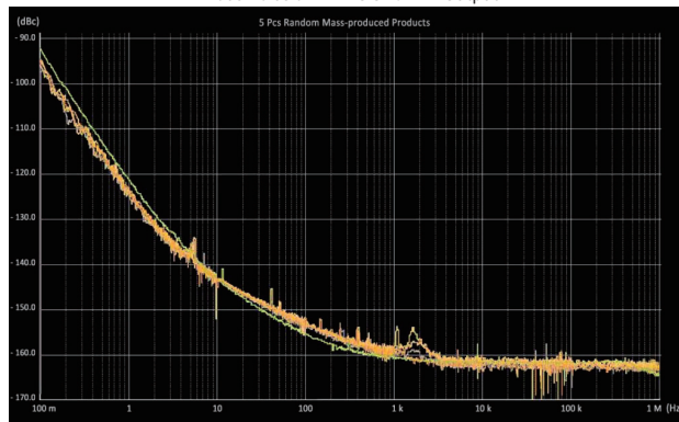
Phase Noise of NADAC C 10 MHz Output
